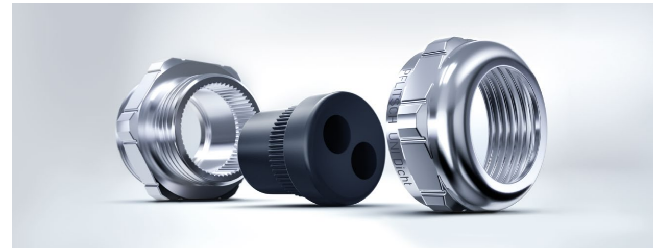
UNI Dicht cable gland with multiple sealing insert
